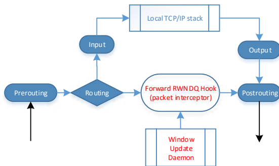
Figure 3: NetFilter-based RWNDQ packet processing pipeline
