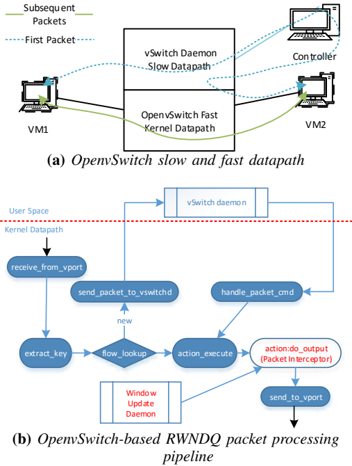
Figure 7: RWNDQ OpenvSwitch-based implementation
